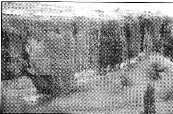
Photo 5 - Le Beaumier, Coirons.
